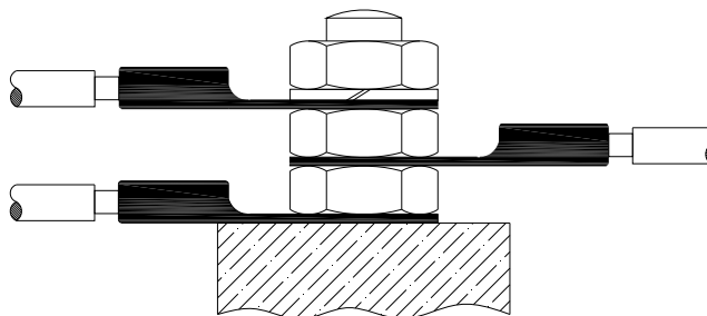
Figure 2: Earth connection
